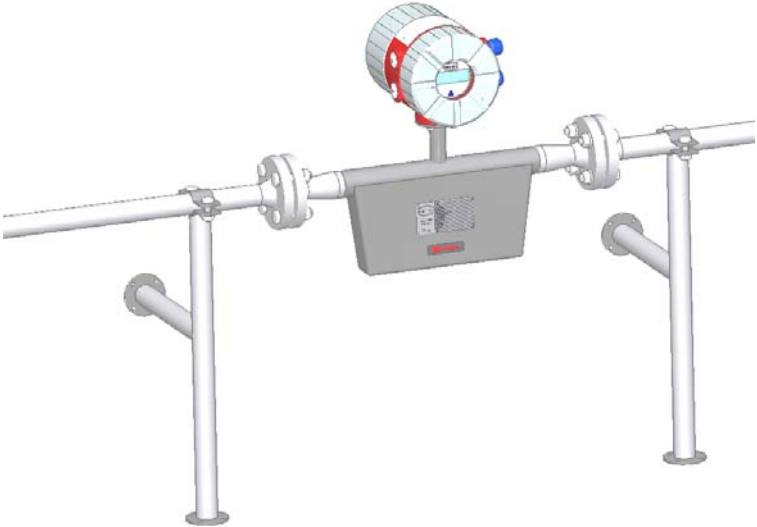
Foot-mounted installation
