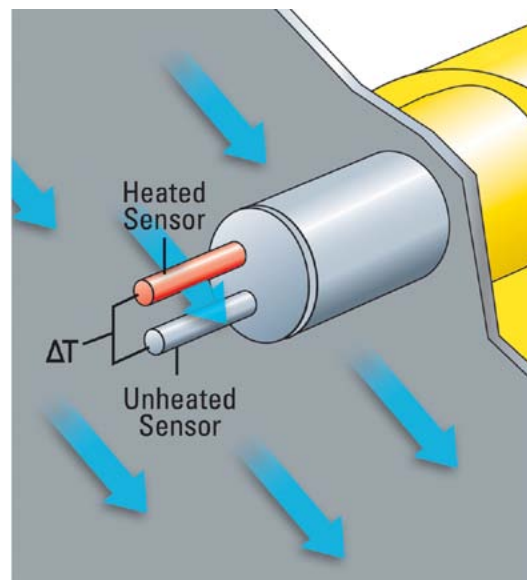
Figure 3: Thermal dispersion constant power principle of operation
