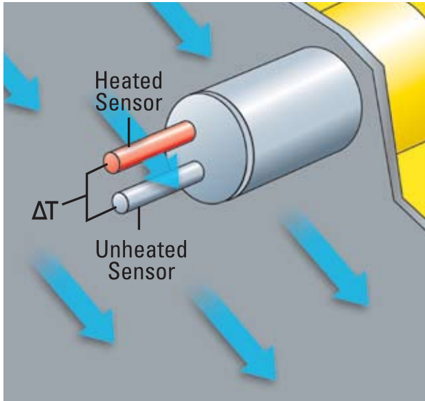
Figure 2. Thermal Mass Flow Sensing Theory of Operation
