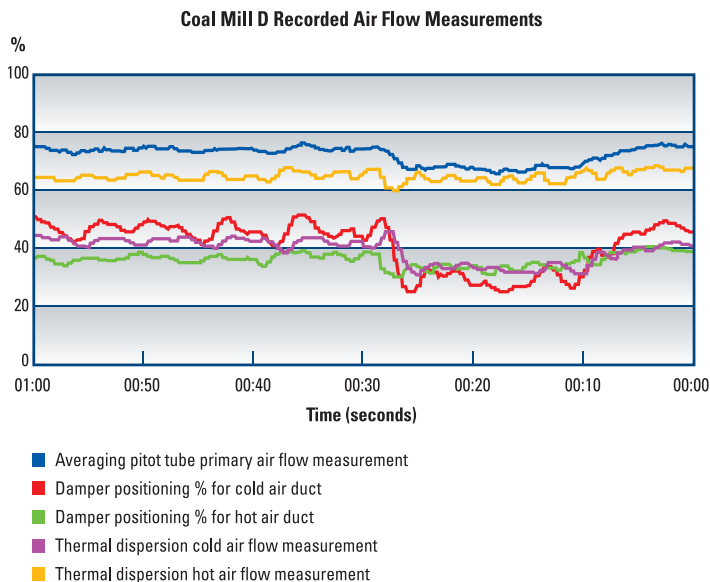
Figure 5: Test data for thermal mass flow meter
